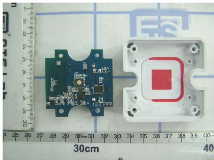
Figure 4 (Internal view -2)
