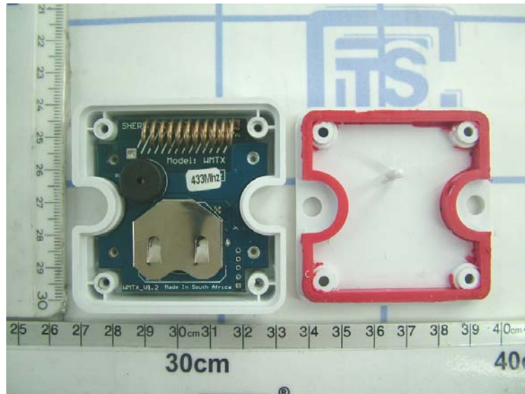
Figure 3 (Internal view -1)
