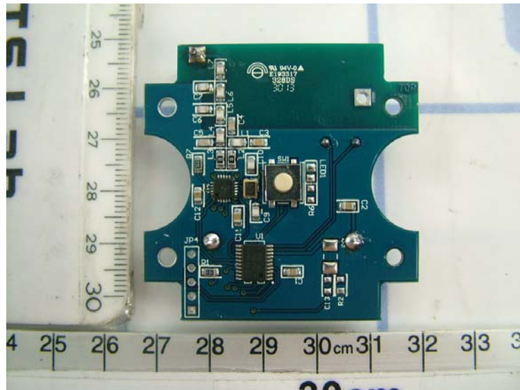
Figure 5 (PCB –side 1)
