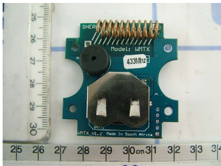
Figure 6 (PCB –side 2)
