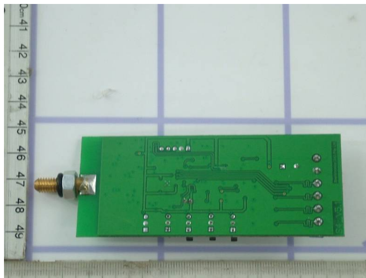
Figure 6 (Transmitter, PCB –side 2)
