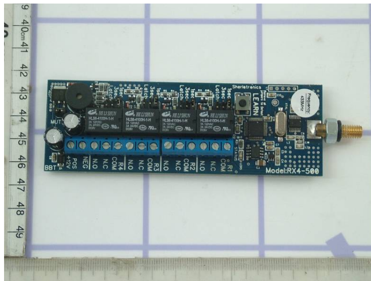
Figure 10 (Receiver, PCB -side 1)
