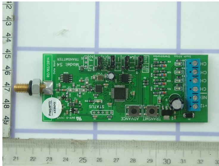
Figure 5 (Transmitter, PCB –side 1)
