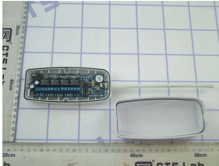
Figure 9 (Receiver, Internal view)
